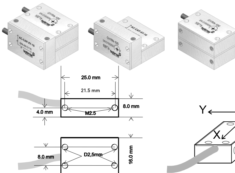
AC-CAP1 1 axis spec V04
